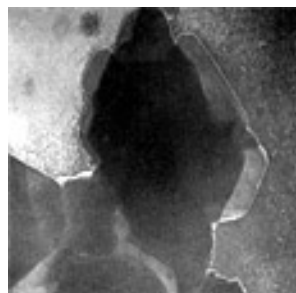
Platelets
